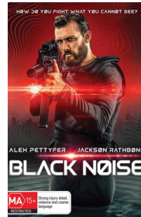
Black noise
