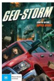
Geo-storm
